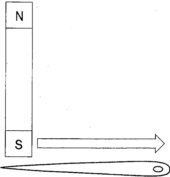
MAGNETIZATION
