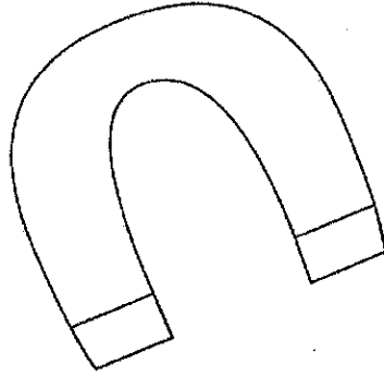
Permanent Magnet
