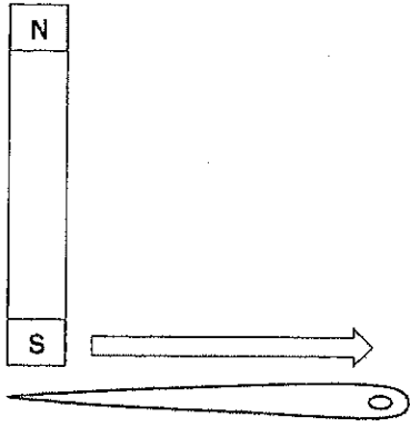
Temporary Magnet
